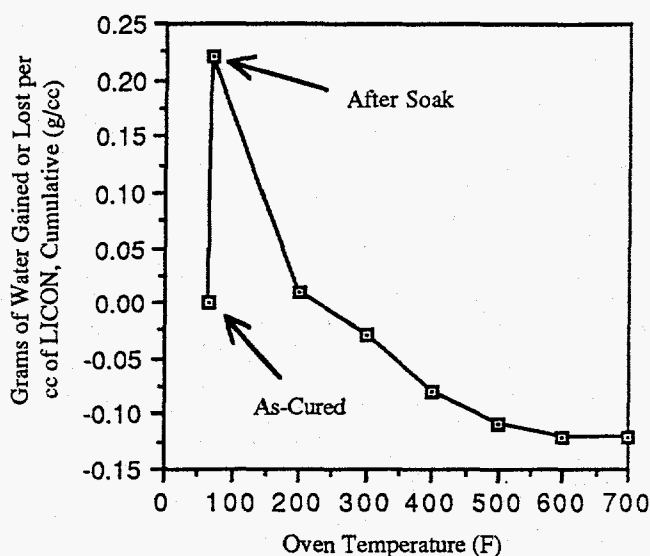
Figure 7. Weight Gained/Lost per cm 3 of LICON as a Function of Temperature.
