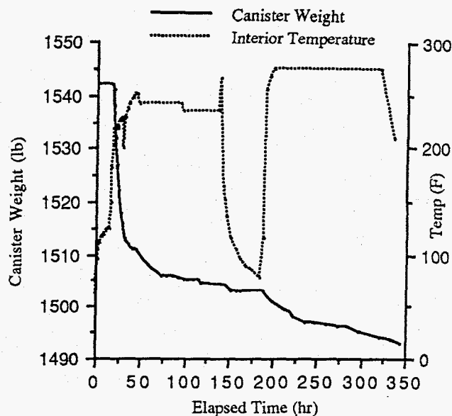
Figure 2. Empty Canister Drying.
