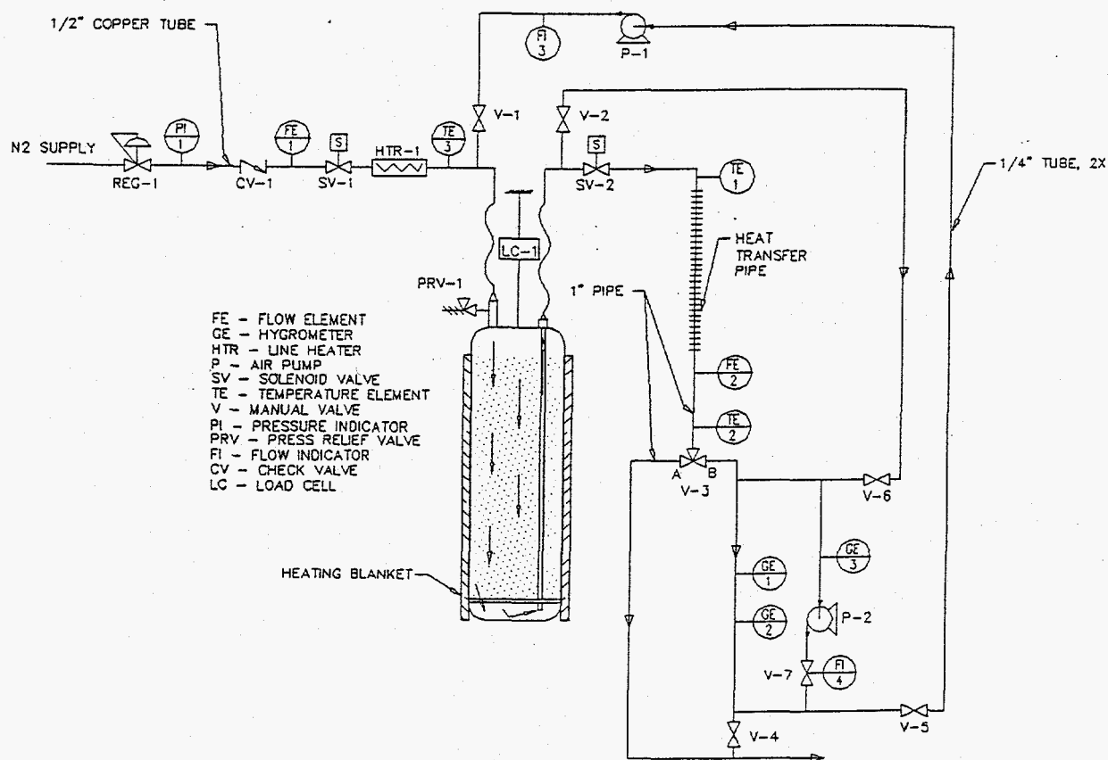
Figure 1. Piping and Instrumentation Diagram for Drying Tests.
